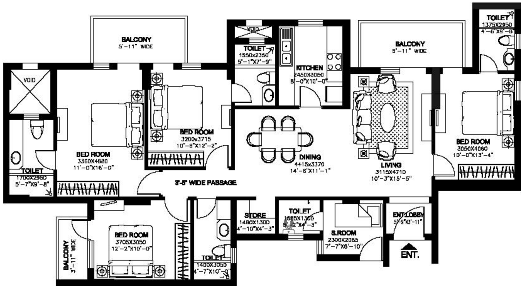
TENTATIVE PLAN OF APARTMENT NO. 3 & 4 IN BLOCK A, B, C & D
